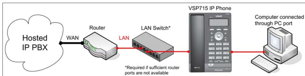
Figure 1. VSP725 Installation Example
